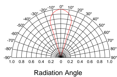
Radiation Characteristics
