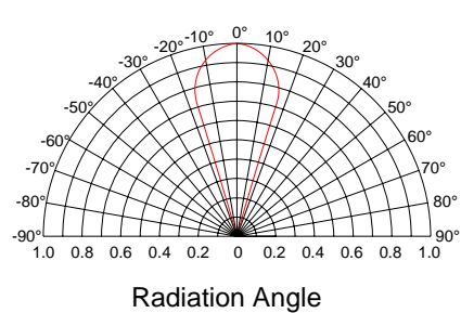
Radiation Characteristics
