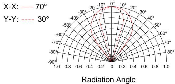
Radiation Characteristics
